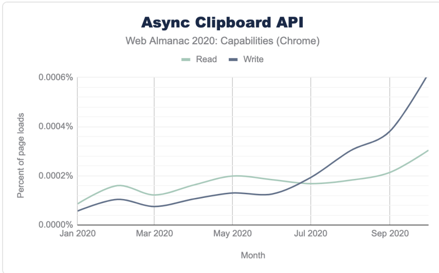
Figure 13.1. Percentage of page loads in Chrome using Async Clipboard API. (Sources: Async Clipboard Read 544 , Async Clipboard Write 545 )
