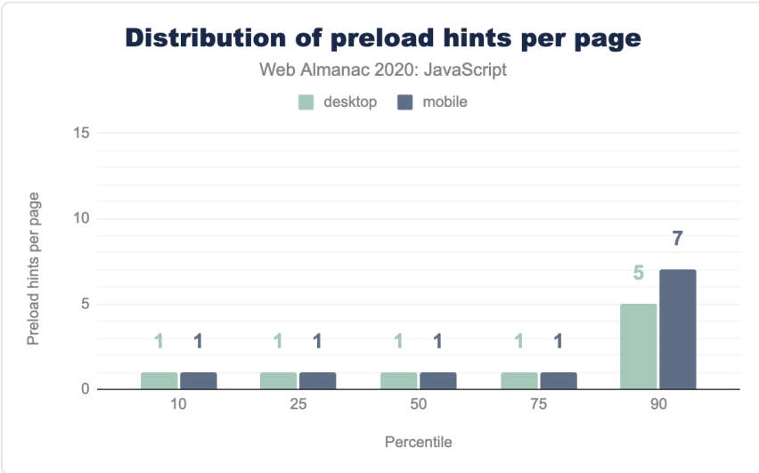
Figure 2.15. Distribution of the number preload hints per page with any preload hints.
